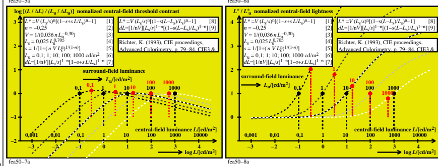
TUB-test chart fea5; Achromatic thresholds; 5 luminances L_u=0,1, 1, 10, 100, 1000 cd/m 2 , with L_m \Delta L (0,4s) , contrast, and lightness; experimental data of Lingelbach and equations of Richter
