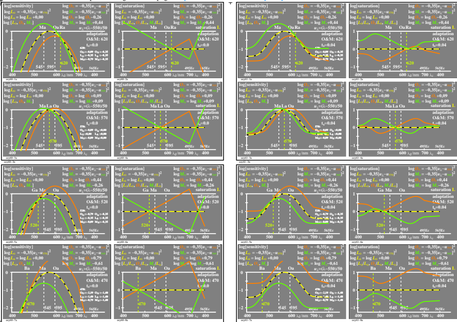
TUB-test chart ey6; sensitivity LMO→M/L & O/L, lin[thresholds]=0 & 0.04 log[sensitivity] and log[ratio], LMS-R21, 4 adaptations: 620,570,520,470
