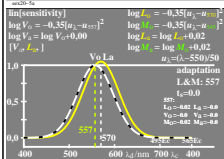
TUB-test chart ex2; sensitivity LMV→L/V & M/V, lin[thresholds]=0 & 0.04 lin[sensitivity] and lin[ratio], LMS-R21=570,545,557, adaptation 557
