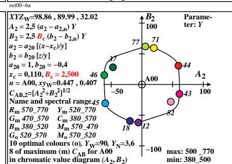
TUB-test chart eet0; Ostwald optimal colours, Yw=90 & 100, D65, D50, P40, A00, CIE-02-degree Antagonistic hue circle, approximately constant chromatic value CAB,2 for contrast C=>288:1
