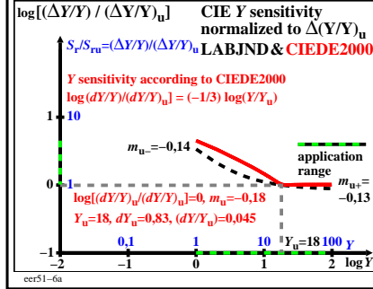
TUB-test chart eer5; Comparison of the LABJND and the CIEDE2000 colour-difference formula log[lightness L*, threshold ΔY, sensitivity ΔY/Y, contrast Y/ΔY, unnormalized and normalized]
