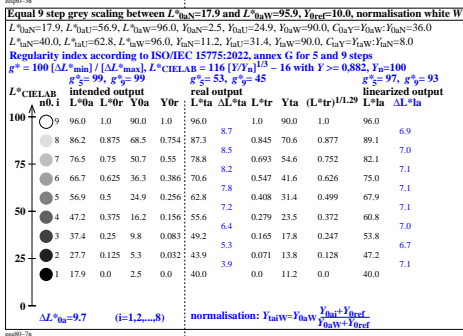
Test chart eq8; Equal 9 step grey scaling for four display reflections Y_{ref}=2.5, 10, 20, 90 , and black L^*_{N,CIElab}=17.92 , Y_N=2.5 and white L^*_{W,CIElab}=95.99 , Y_W=90 , normalisation: white W
