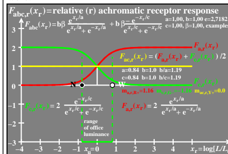
TUB-test chart een5; TUBJND model, lightness F_{abc} , F_{abc,r} , receptor responses F_{ab}(R^+) , F_{cb}(G^-) , F_{ab}+F_{cb}(Y^+) (left), relative responses (right) for equal parameters a and b
