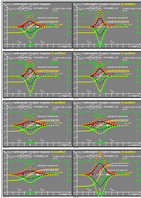
TUB-test chart eej5; TUBJND model of response functions F_{ab}(x_r) , and derivation F'_{ab}(x_r) Receptor responses R+, G-, Y+, and derivations Y+', Y-' (left & right), and R+', G-' (right)
