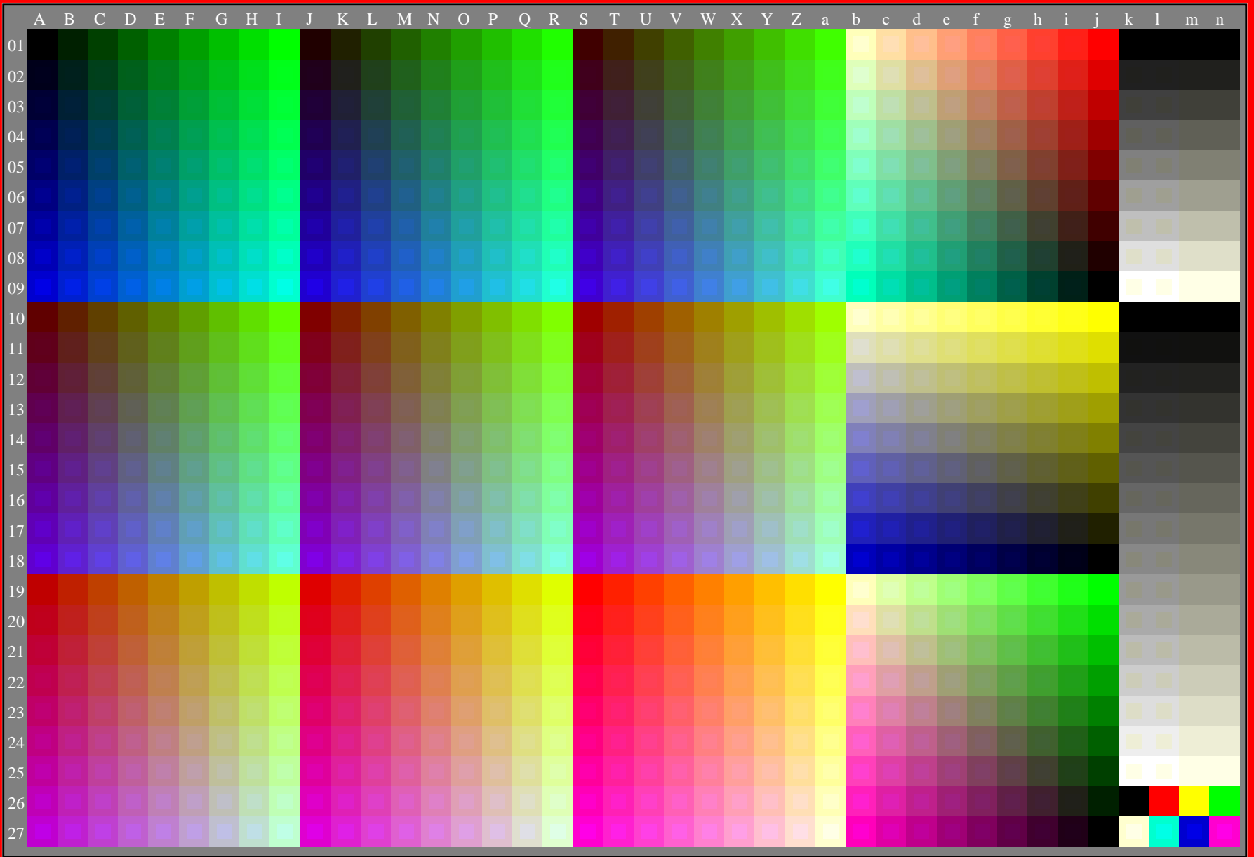
eei90-8A, gamma g_a=2,400 , g_p=1,000 , C_{YP8}=C_{YN8} , Yellow colour tint
