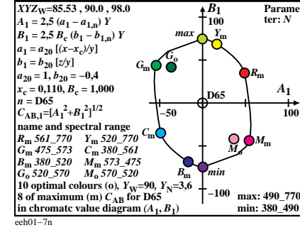
TUB-test chart eeh0; Ostwald optimal colours, Y_N=3,6 , Y_W=90 , illuminant D65, CIE-02-degree Ostwald optimal colour data: XYZ and eight different colour diagrams,
