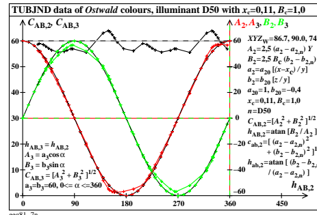
TUB-test chart eeg8; CIEXYZ and TUBJND data of the hue circle of the Ostwald colours for CIE standard illuminant D50 with x_c = 0,11 and B_c = 1,0 , hue angle difference \Delta h_{ab,2} variable
