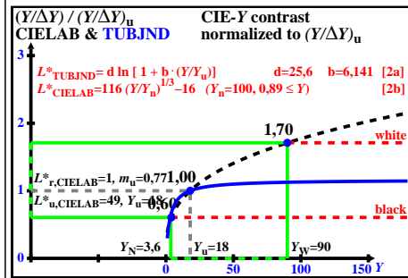
TUB-test chart eef9; Contrast (Y/\Delta Y) / (Y/\Delta Y)_u = f(Y) of colour spaces CIELAB & TUBJND, see ISO/CIE 11664-4 & CIE 230, many information (left), and less (right)
