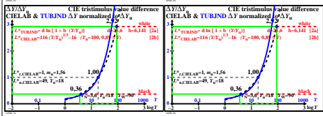
TUB-test chart eef4: CIE tristimulus value difference \Delta Y/\Delta Y_u = f[\log(Y)] of colour spaces CIELAB & TUBJND, see ISO/CIE 11664-4 & CIE 230, many information (left), and less (right)
