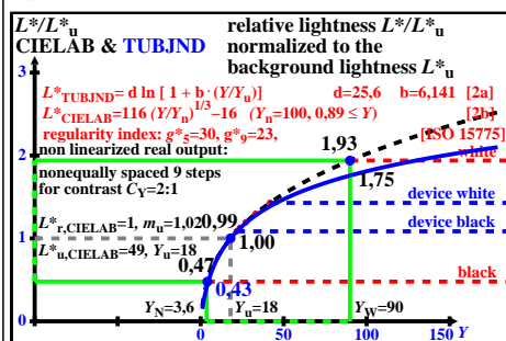
TUB-test chart eef3; Relative lightness L^*/L_u^* = f(Y) of colour spaces CIELAB & TUBJND, see ISO/CIE 11664-4 & CIE 230, many information (left), and less (right)
