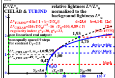
TUB-test chart eef3; relative lightness L^*/L^*_u = f(Y) of colour spaces CIELAB & TUBJND; see ISO/CIE 11664-4 & CIE Z30, many information (left), and less (right)
