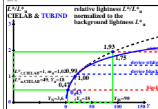
TUB-test chart eef3; relative lightness L^*/L^*_u = f(Y) of colour spaces CIELAB & TUBJND; see ISO/CIE 11664-4 & CIE Z30, many information (left), and less (right)
