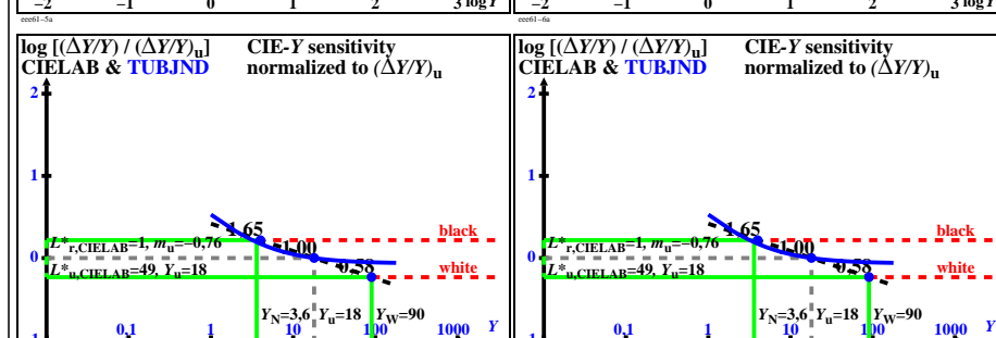
TUB-test chart eee6; Sensitivity \log[(\Delta Y/Y) / (\Delta Y/Y)_u] = f[\log(Y)] of colour spaces CIELAB & TUBJND, see ISO/CIE 11664-4 & CIE 230, many information (left), and less (right)
