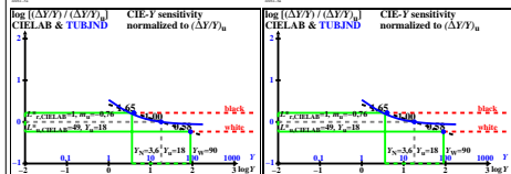
TUB-test chart eee6; Sensitivity \log[(\Delta Y/Y) / (\Delta Y/Y)_u] = f[\log(Y)] of colour spaces CIELAB & TUBJND, see ISO/CIE 11664-4 & CIE 230, many information (left), and less (right)
