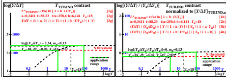
TUB-test chart ea6; TUBJND colour space and colour differences, see CIE 230:2019 log(lightness L*, threshold ΔY, sensitivity ΔY/Y, contrast Y/ΔY), unnormalized and normalized for U
