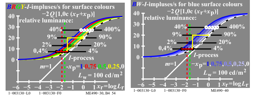
Fig. 54: Colour signals of chromatic and blue colours
