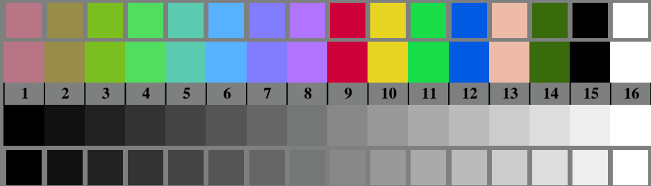
DEE00–7, Picture B3: 14 CIE-test colours according to CIE 13.3 and 16 grey steps
