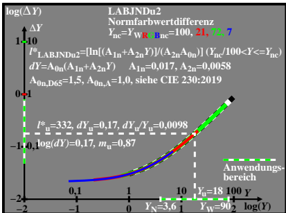
CGH20-3A
