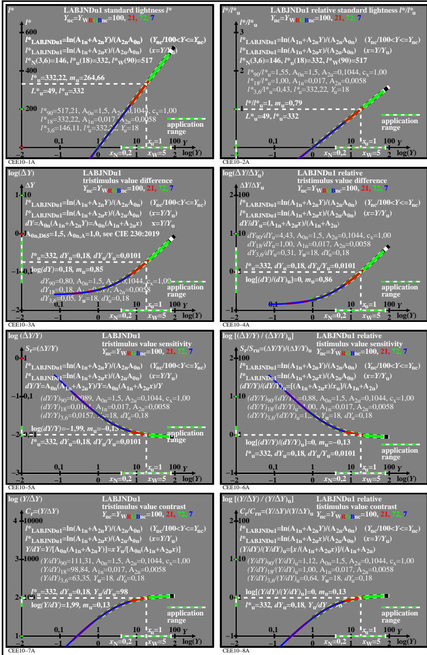
TUB-test chart CEE1; LABJNDu1, l^*(Y) & L^*(Y) , Y_{nc}=(Y \cdot L^*)_{Wnc} , c_x=1,00 , with more data Absolute and relative lightness, sensitivity and contrast, A_{0n}=1,5, A_{1n}=0,017, A_{2n}=0,0058, A_{2u}=0,104
