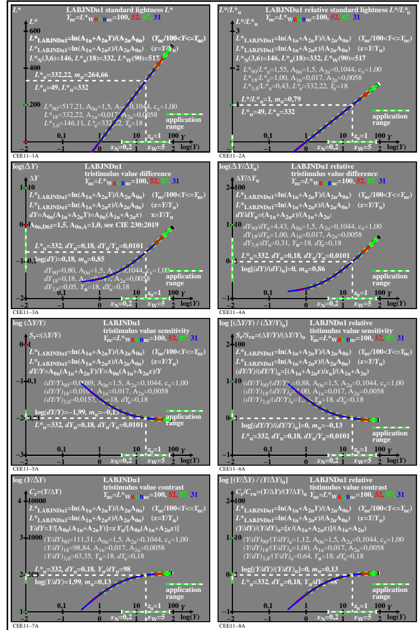
TUB-test chart CEE1; LABJNDu1, l^*(Y) & L^*(Y) , Y_{nc}=(Y \cdot L^*)_{Wnc} , c_x=1,00 , with more data Absolute and relative lightness, sensitivity and contrast, A_{0n}=1,5, A_{1n}=0,017, A_{2n}=0,0058, A_{2u}=0,104
