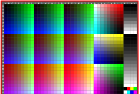
ADW91-5A, gamma g_a=2,400 , g_p=1,000 , C_{Y12}=C_{Y14}
